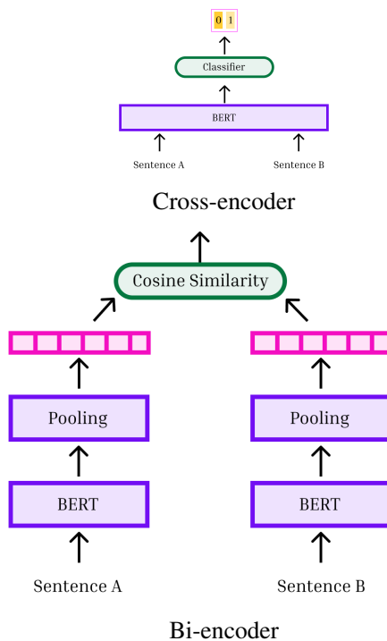
FIGURE 6. ARCHITECTURES TO COMPARE TEXTS.
