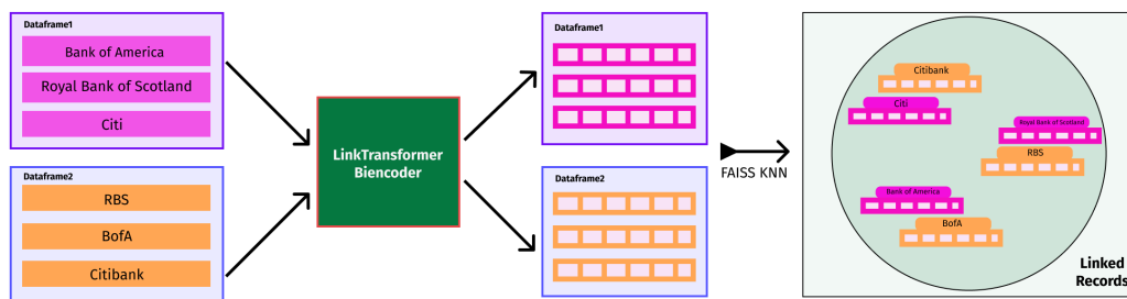
FIGURE 8. LINKTRANSFORMER ARCHITECTURE.
